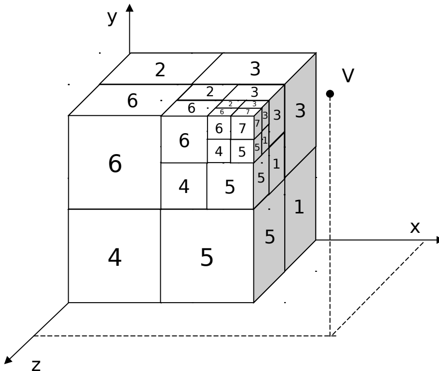
Back to front enumeration and visible faces
